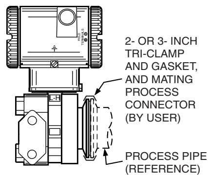
MODEL PSSCT FLUSH DIAPHRAGM SANITARY SEAL WITH TRI-CLAMP
